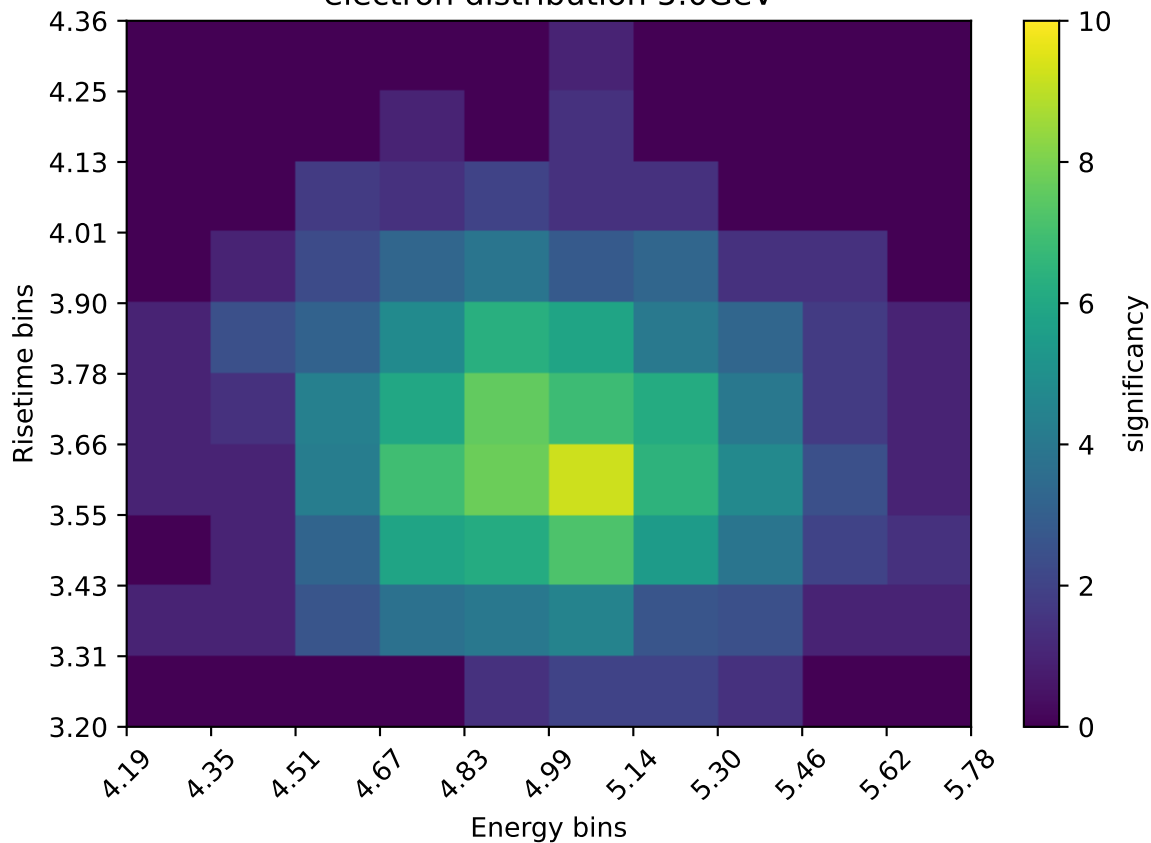
electron distribution 5.0GeV
